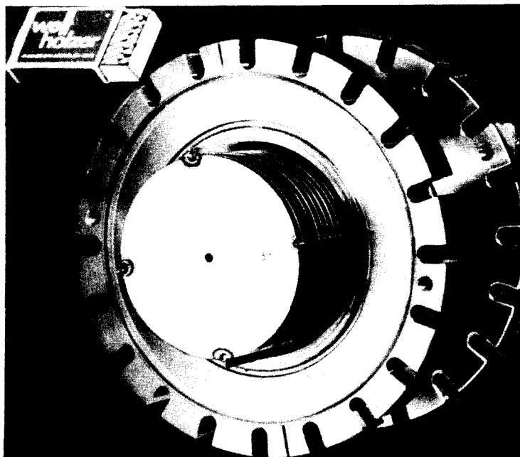
Fig. 12. Wake field transformer: (a) The photo displays slices which are held together by metal strips forming a stack lying normally inside the tube. On the inner wall of this tube are ring shaped channels in which the wake fields are excited by the driving hollow beam. The wake fields are guided by the slices into the center of the tube where they interact with the driven beam. All parts are made from stainless steel. (b) Sectional drawing of a part of the wake field transformer.
