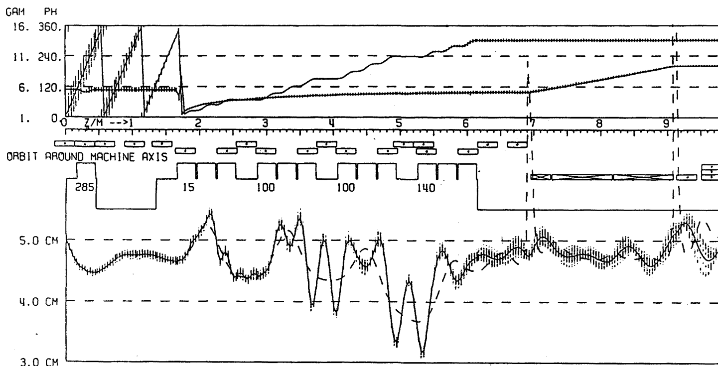
Fig. 11. Typical plot output of the WAKTRACK tracking code, showing several particle properties in the DESY experiment. In the middle between the two frames, a scheme of the experimental set up is drawn, together with a scale, which can be compared to figure 1. The coils are sketched and near the cavity contours their phases are written in degrees. Below this, the orbit of the particles is plotted: the ring radius varies between 3 and 5 cm due to transverse forces at gaps between coils and in cavities. The collective oscillation around the dashed reference orbit is reduced in its amplitude by adjusting the current in the coils between the third and the fourth cavity ( 4.6 \text{ m} < z < 5.6 \text{ m} ). Above the set up sketch two curves are plotted in one frame, the relativistic \gamma factor and the phase difference compared to a particle moving with the speed of light. In front of the first accelerating cavity ( z < 1.7 \text{ m} ), where the particles are nonrelativistic, (\gamma - 1) is stretched by a factor of 30. Behind that, the increasing energy in the linac can be seen. The phase difference of nonrelativistic particles changes with a certain slope depending on the particle velocity. When the particle speed approaches c , the phase becomes constant. It only changes again in the high energy buncher ( 7 \text{ m} < z < 9 \text{ m} ), where the velocity parallel to the z -axis is decreased by rotating the hollow beam.
