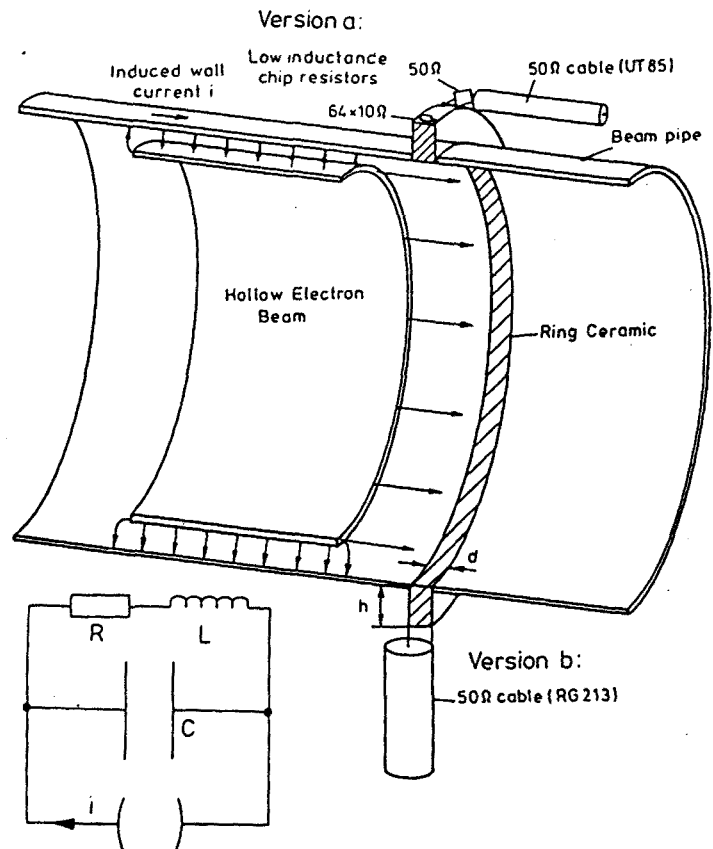
Fig. 6. Physical layout and wiring of the gap monitor at the low energy end of the linac (Version a) and its equivalent circuit ( L = 50\text{pH} , C = 50\text{pF} and R = 0.156\Omega ), which can explain the observed oscillations of about 3 GHz between the bunches (see fig. 5). (Version b) Short connection from the ceramic ( d = 4\text{mm} , h = 7\text{mm} ) to one of the 32 big 50\Omega cables damping the oscillations occurring at the high energy end aperiodically.
