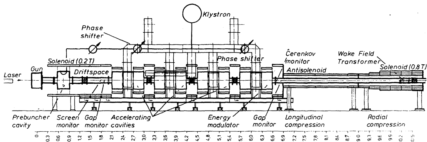
Fig. 1. Overall layout of the Wake Field Transformer experiment at DESY shown from left to right: The infrared light beam produced by a Q-switched Nd-Yag laser (peak power > 100\text{ MW} ) is focused on a ring shaped tantalum cathode. The emitted thermionic- and photoelectrons are extracted by a voltage of about 100 kV and guided by solenoid fields of 0.2 T into the linac. First the hollow beam becomes compressed longitudinally in a prebuncher. Then four 3-cell cavities (500 MHz) accelerate it to 8 MeV. A pulsed klystron (peak power 1 MW) feeds the cavities. In the antisolensoid further longitudinal compression is achieved. By increased solenoidal fields at the end radial compression takes place too. After that the electron ring enters the actual Wake Field Transformer, consisting of 80 cylindrical cells arranged one after another. For monitoring and adjustment of the ring beam, several beam monitors have been set up.
