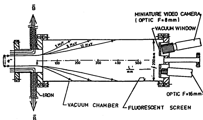
Fig. 10. Hollow beam spectrometer making use of the end field of the solenoid on the left side (not shown). By an iron sheet (3 cm thick) the inner longitudinal field is bent outwards within a short range. Here the passing electrons experience a transverse momentum and hit the fluorescent screen at the inner wall of the spectrometer tube at a longitudinal position corresponding to their energy.
