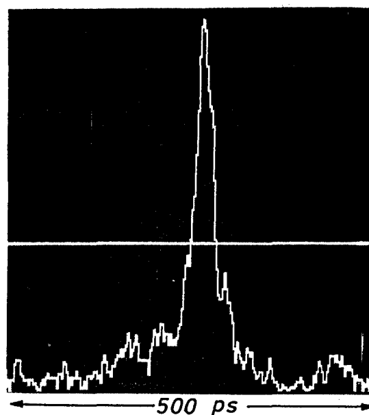
Fig. 9. Single bunch signal taken with the streak camera. The width (FWHM) corresponds to a length of 1 cm.
