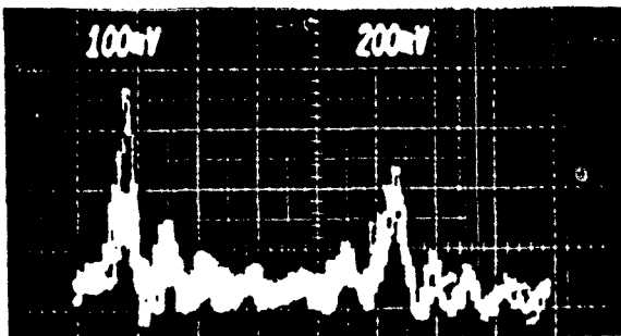
Fig. 5. Two of 5 bunches produced by a single laser shot. The separation between them is 2 ns. The bunch length is about 150 ps (FWHM). The signals are produced by a gap monitor in front of the linac behind a drift space of 1.2 m after the end of the prebuncher cavity. They are detected by a sampling oscilloscope.
