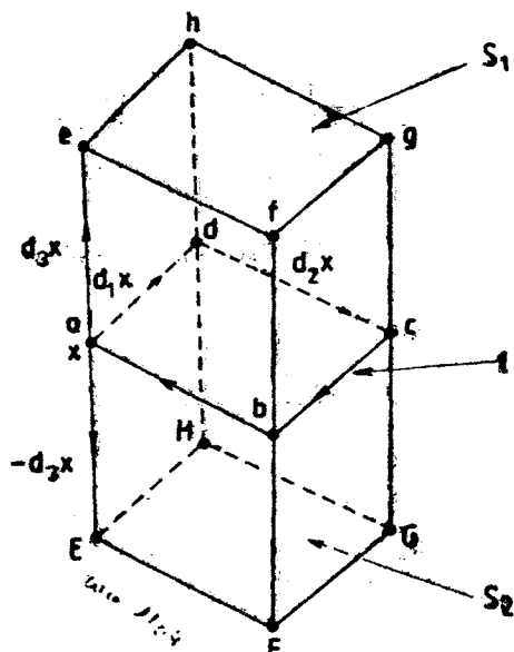
Fig. 3. Two surfaces having common edge \partial S_1 = \partial S_2 = l
