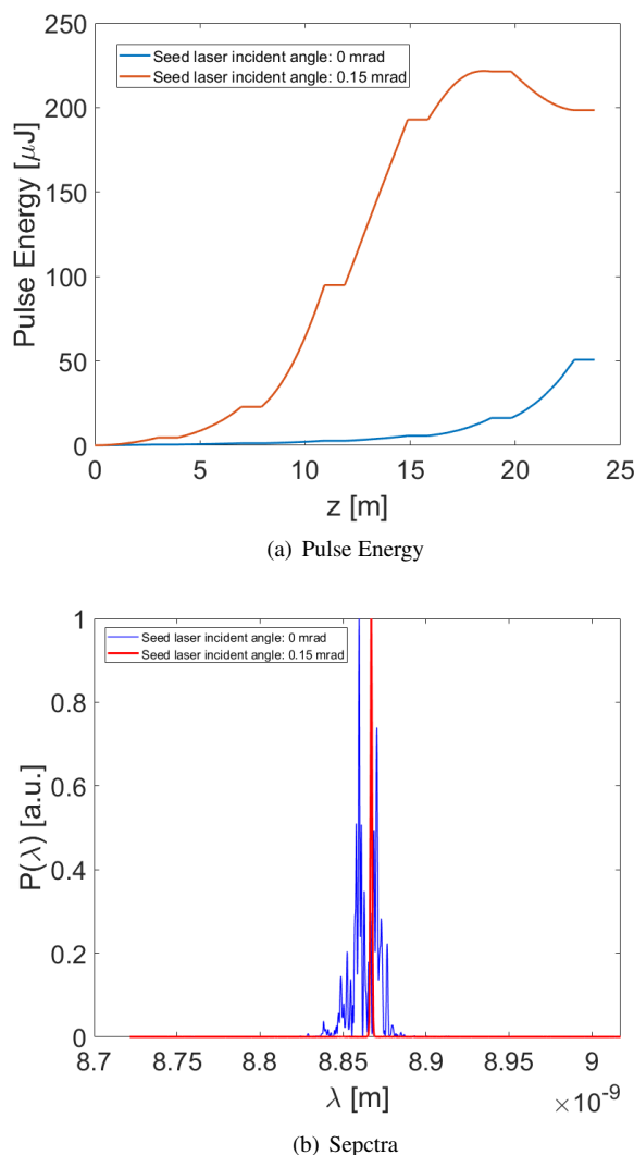
Figure 5: The pulse energy (a) and spectra (b) comparison for FEL radiation results with 0.15\text{ mrad} incident angle and straight incident.
