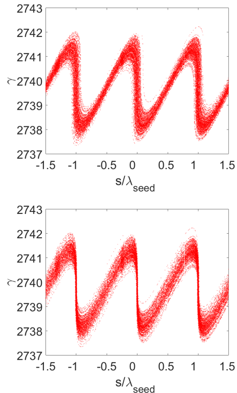
Figure 3: Typical HGHG effect with straight incident seed laser (top) and PEHG effect with oblique incident seed laser (bottom).
