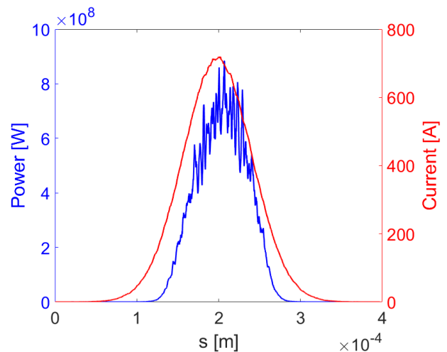
Figure 4: PEHG-FEL radiation.
