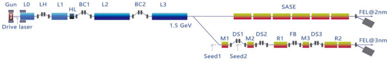
Figure 2: The schematic layout of the SXFEL user facility.
