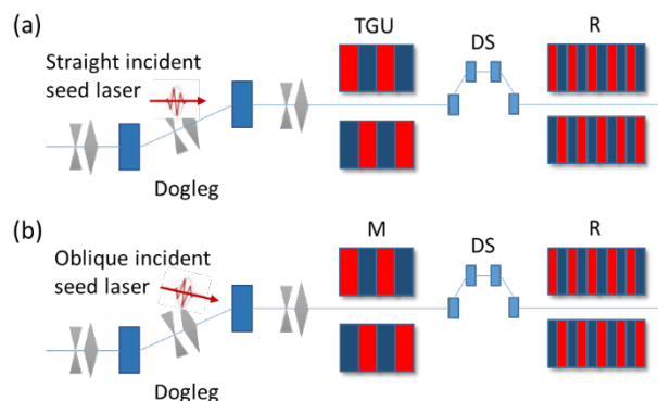
Figure 1: Two different PEHG schemes.
