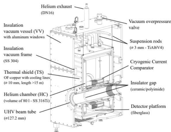
Figure 2: Schematic of CCC beam line cryostat, with its main components highlighted.
