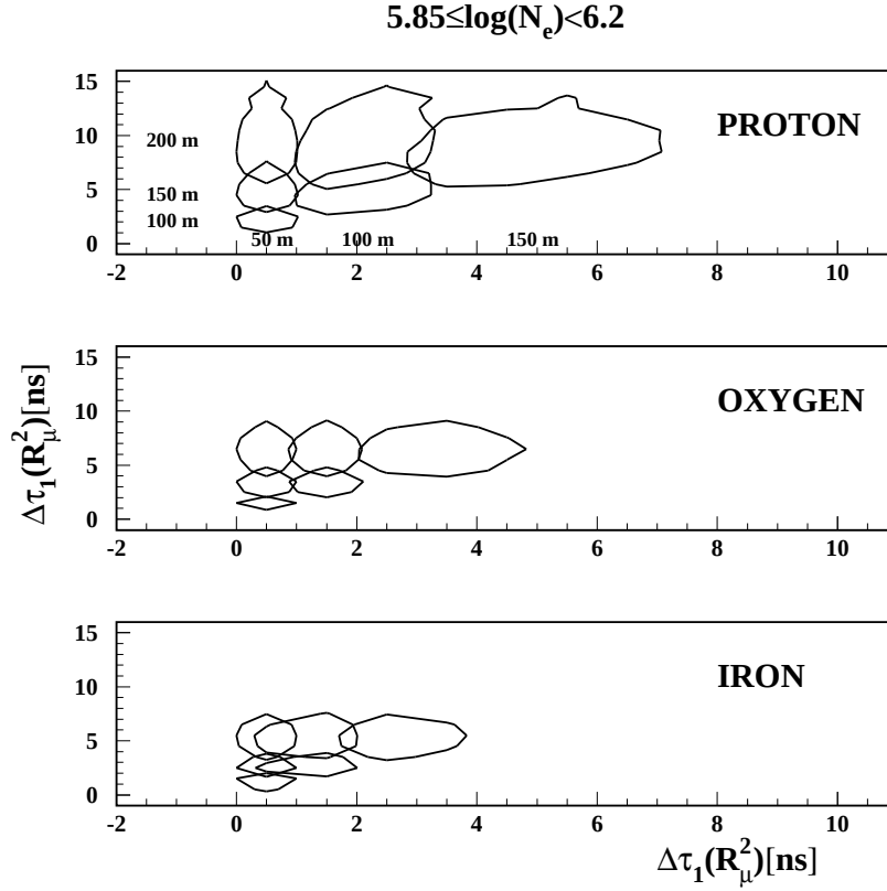
Fig. 2. Half-maximum contours of the distributions of correlated muon arrival time observed at different distances from the shower core for different types of primaries [4].
