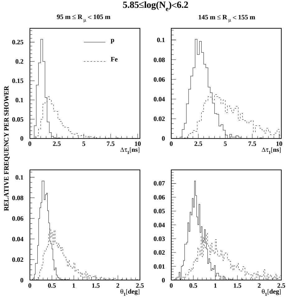
Fig. 1. Single muon time arrival and angle-of-incidence distributions corresponding to R_\mu = 100\text{m} si R_\mu = 150\text{m} for different primaries.
