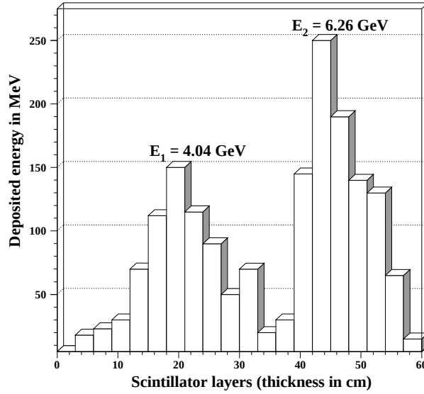
Fig. 3. Two cascades measured in a real event producing two secondaries with kinetical energy 4.04 GeV and 6.26 GeV, respectively.
