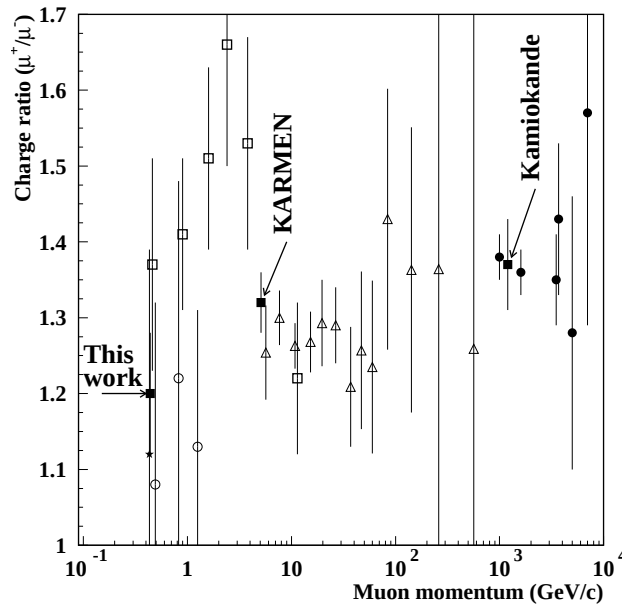
Fig. 4. Compilation of muon charge ratio results: \square Allkofer et al.(1972), \triangle Nandi et al.(1972), \bullet Utah (1972), \circ MASS2 (1991), \star IMAX(1992)
