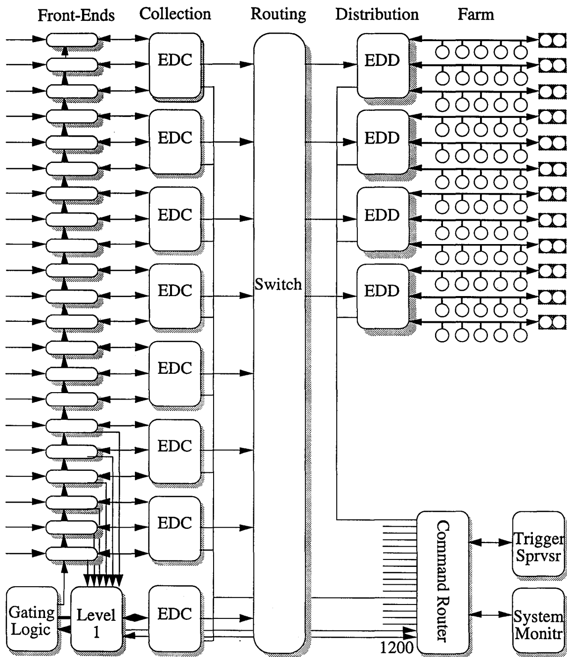
Fig. 1. GEM data acquisition architecture.
