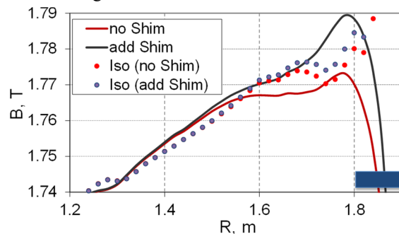
Figure 6: Magnetic fields at the area of extraction radius with and without valley shims, are shown by lines. Circles present corresponding isochronous fields. Blue rectangle shows the radial position of the valley shim.
