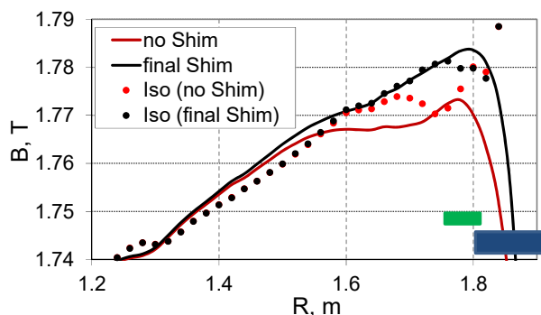
Figure 8: Magnetic field with and without final shimming, are shown by lines. Circles represent corresponding isochronous fields. Green and blue rectangles show sector and valley shims radial position.
