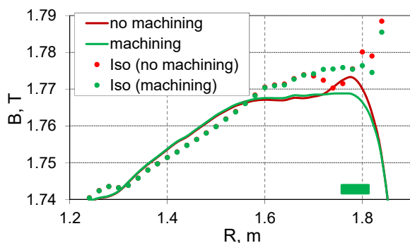
Figure 7: Magnetic fields at the area of extraction radius with and without shim machining, are shown by lines. Circles present corresponding isochronous fields. Green rectangle shows radial position of sector shim machining.
