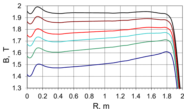
Figure 4: U400M magnetic field at operative levels.
