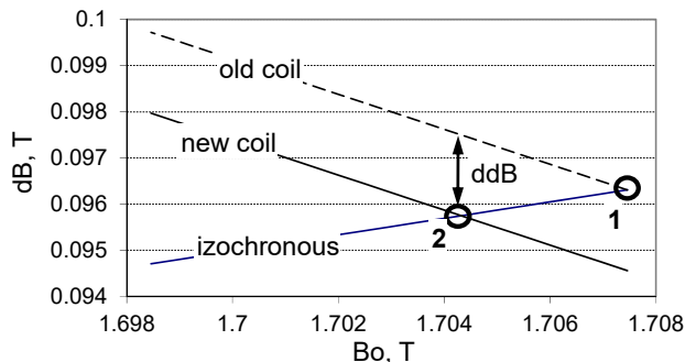
Figure 3: Changing of magnetic field level for operation mode A/Z = 3 with new coil.
