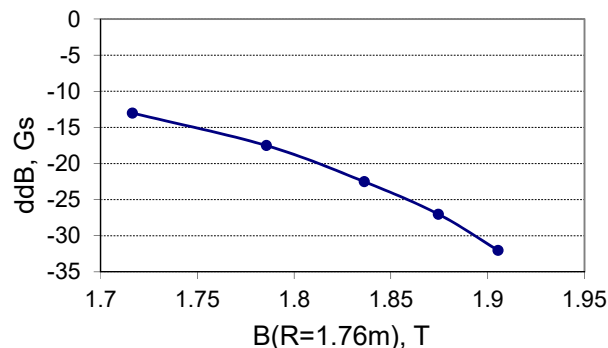
Figure 2: The change of magnetic field radial growth because of main coil reconstruction.
