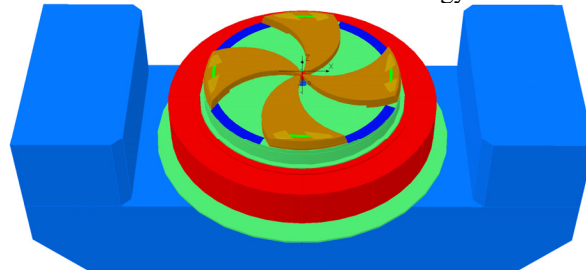
Figure 5: Computer model of U400M magnet with additional valley shims and machining of sector shims.
