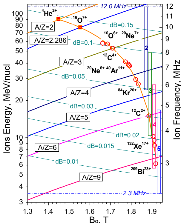
Figure 1: The operation modes diagram of U400M.
