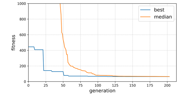
Figure 3: The process of optimization with DE algorithm.
