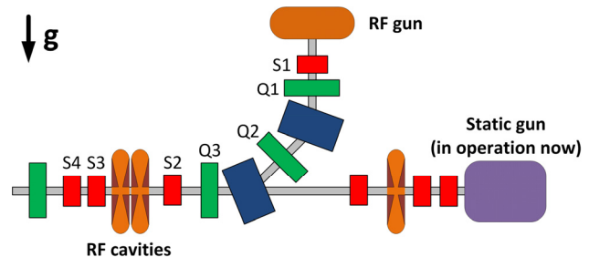
Figure 1: A scheme of the NovoFEL injector with the new RF gun: red – solenoids, green – quadrupoles.
