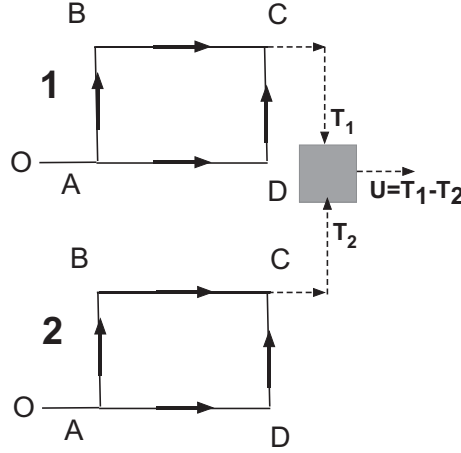
Fig. 2. – Diagram of the double atom interferometer.
