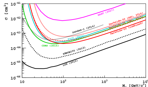
Figure 4. Spin-independent WIMP-nucleon cross section 90 % C.L. exclusion plot for DarkSide-50, compared to other experiments. See Ref. [2] for a detailed description and references.
