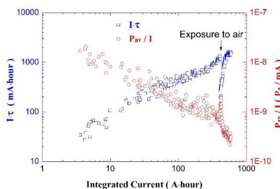
Figure 5: Progress of beam cleaning and growth of beam lifetime.
