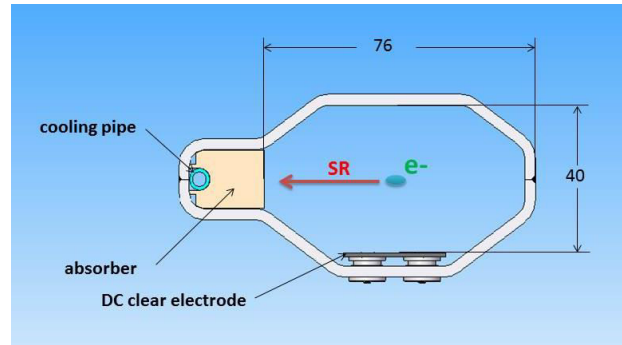
Figure 1: The section of the main vacuum pipe.
