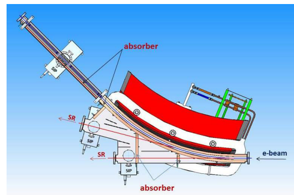
Figure 2: A standard segment of the storage ring.
