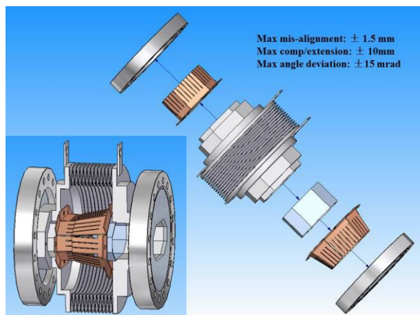
Figure 3: RF shielded bellow.
