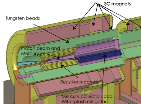
FIGURE 2. Neutrino Factory/ Muon Collider Target Layout.
