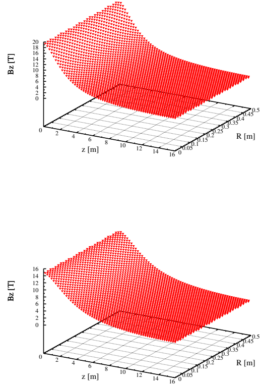
FIGURE 3. 20-T and 15-T target solenoid field maps.
