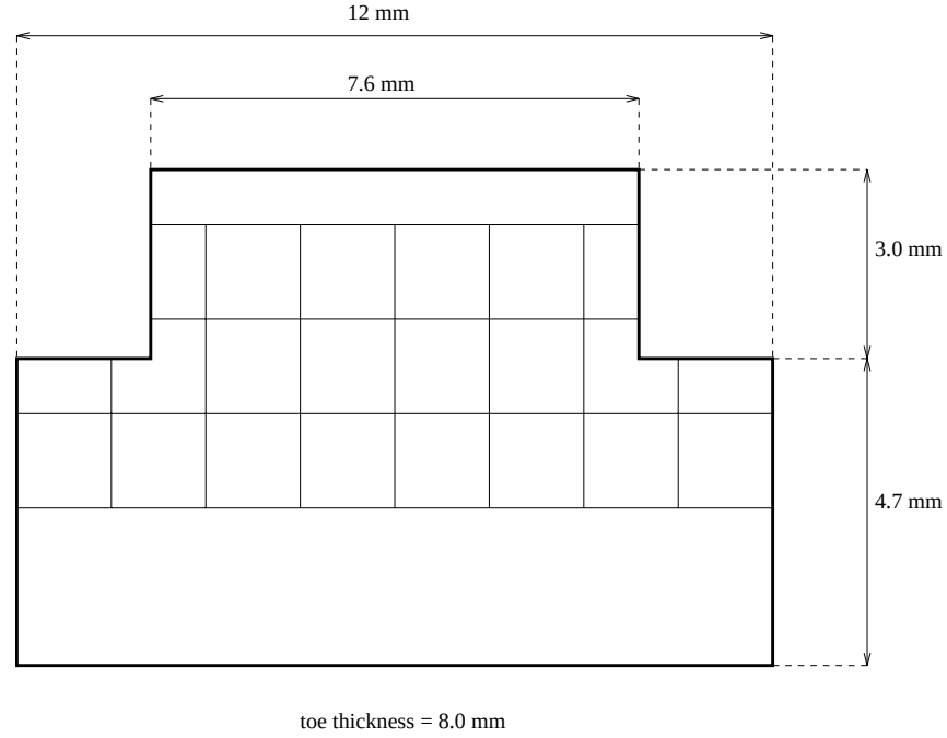
Figure 2.7: Toe counter outline.
