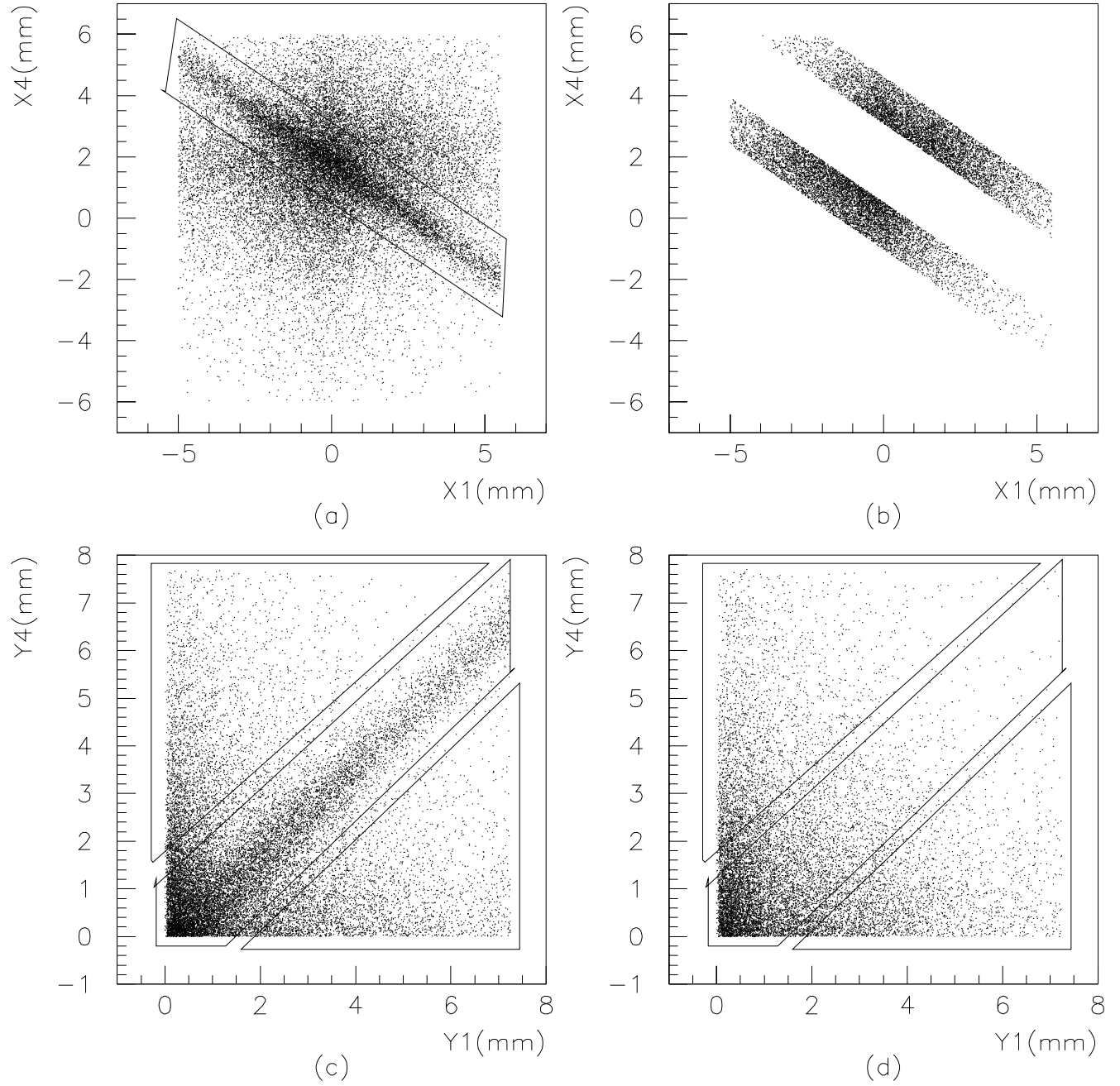
Figure 4.13: YY diagonal events from in \Delta XX and off \Delta XX events. a) cut to get on XX diagonal events. b) off diagonal XX cut. c) YY data from on XX diagonal events. d) YY data from off XX diagonal events. The triangular areas displayed on c) and d) correspond to the data used for normalization.
