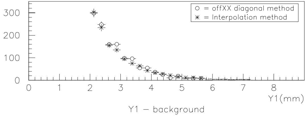
Figure 4.19: Comparison of background measured by the off XX diagonal method and the interpolation method.
