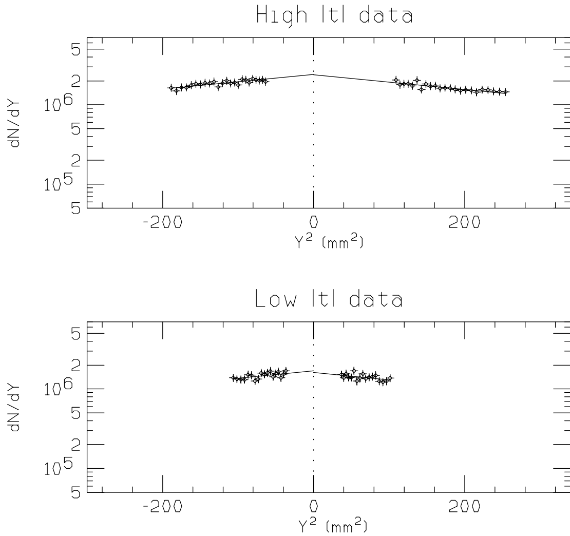
Figure 4.23: \frac{dN}{dY} vs Y^2 distributions for data set 10 (high |t| data) and data set 5 (low |t| data). Data from detector 1 is plotted with Y^2 positive, data from detector 2 is plotted with Y^2 negative.
