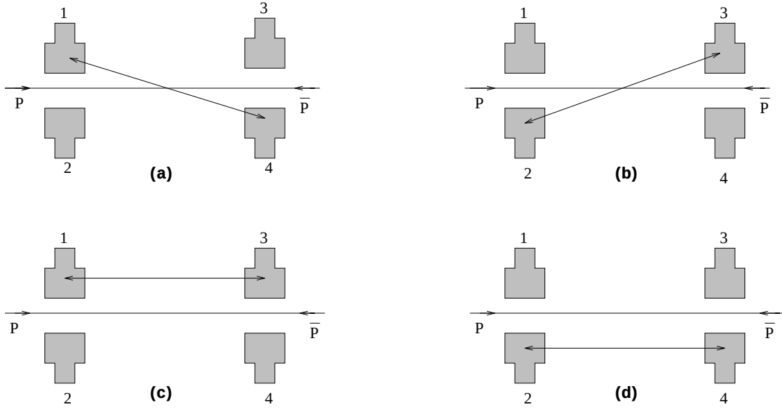
Figure 4.16: OO coincidences. a) and b) are the two elastic combinations. c) is the upper-upper trigger, d) is the lower-lower trigger.
