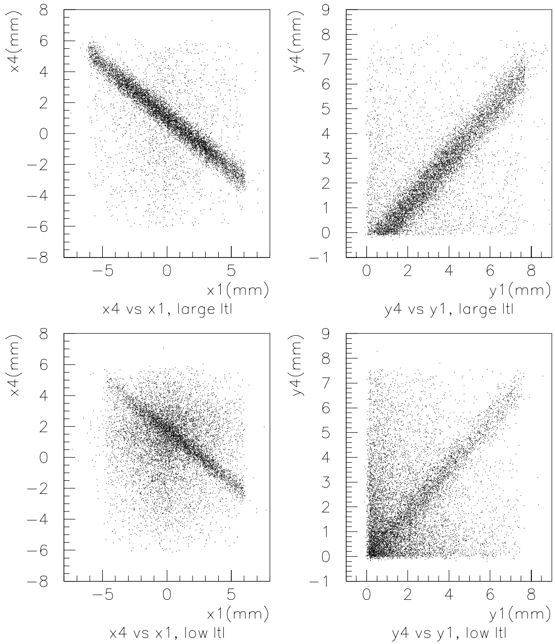
Figure 4.9: XX and YY correlations for elastic events with detectors at two different vertical positions.
