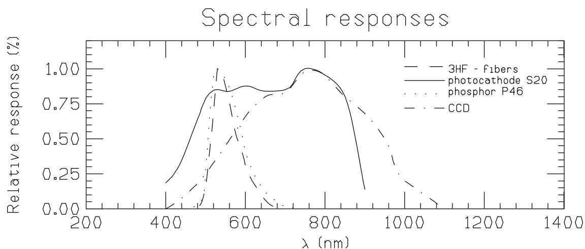
Figure 2.5: Spectral response for different parts of the detector.
