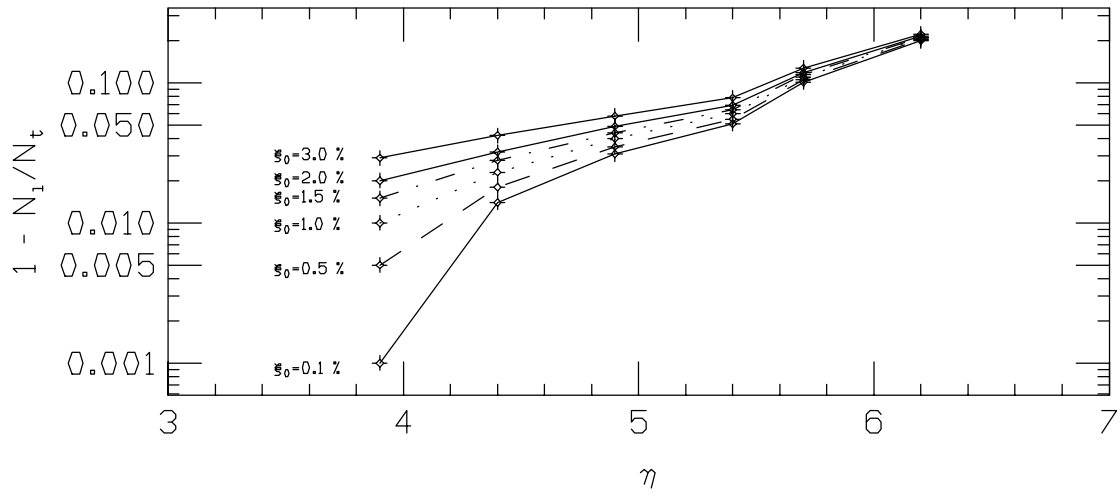
Figure 5.5: Plot of left arm inefficiencies vs \eta for different values of \xi_0 ( \xi_0 =inefficiency of L_{0-5} ).
