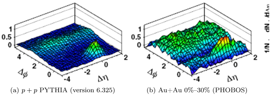
Fig. 3. Two particle correlation function for pp event from PYTHIA MC (left) and central Au-Au collisions at 200 GeV/ c/N from PHOBOS experiment (right) [3].
