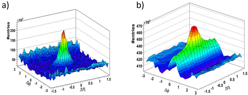
Fig. 2. Two particle correlation function for d -Au (left) and Au-Au central events at 200 GeV/ c/N from STAR experiment [2].
