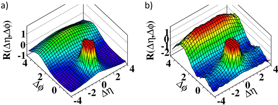
Fig. 1. Two particle correlation function for 7 TeV pp for intermediate p_T range, minimum bias events (left) and high multiplicity events (right). The sharp near-side peak from jet correlations is cut-off in order to better illustrate the structure outside that region [1].
