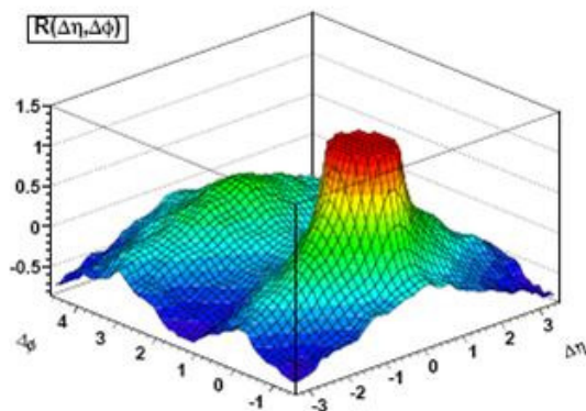
Fig. 5. Two particle correlation function for high multiplicity events in pp collisions at 7 TeV, as obtained from a hydrodynamical evolution based on flux tube initial conditions [10].
