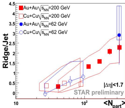
Fig. 4. The Ridge to jet ratio as a function of the number of nucleon participants (centrality measure) from STAR experiment [2].
