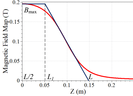
Figure 1: Real fringe field and linear fringe field of a half solenoid.
