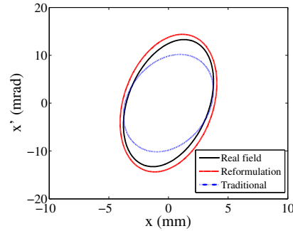
Figure 2: Comparison of the phase spaces at the exit of the exiting half solenoid.
