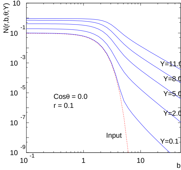
Fig. 1. The amplitude N(r, b, Y) as a function of impact parameter b for different values of rapidity Y . The dipole size and orientation are fixed, r = 0.1 and \cos \theta = 0 . The dashed line is the input distribution (3).
