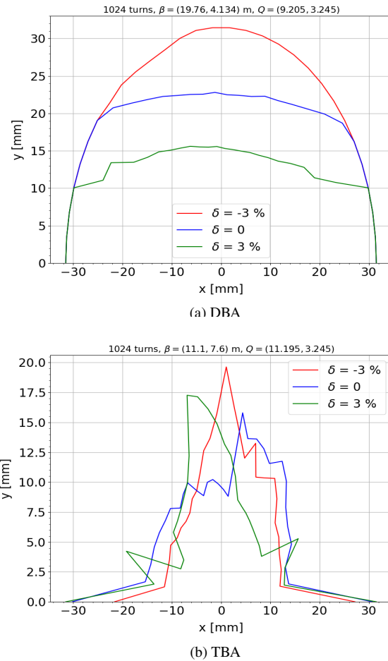
Figure 2: Dynamic aperture for the bare lattices. \delta = \Delta p/p_0 is the momentum offset.
